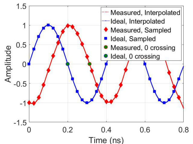
FIGURE 5. Waveform and zero crossing points for measured and ideal signals at 28 GHz.
