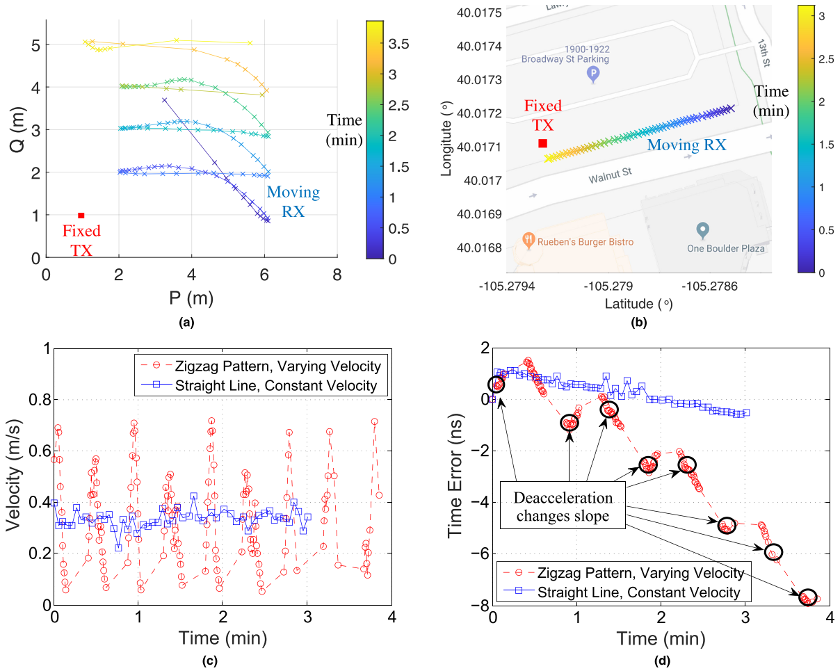
FIGURE 9. Medium-term stability (a) mobile measurement route for zig-zag pattern with varying velocity; (b) mobile measurement route for straight line pattrer with constant velocity; (c) velocity over time for two moving patterns; (d) medium-term timing error as a function of time for two moving patterns.
